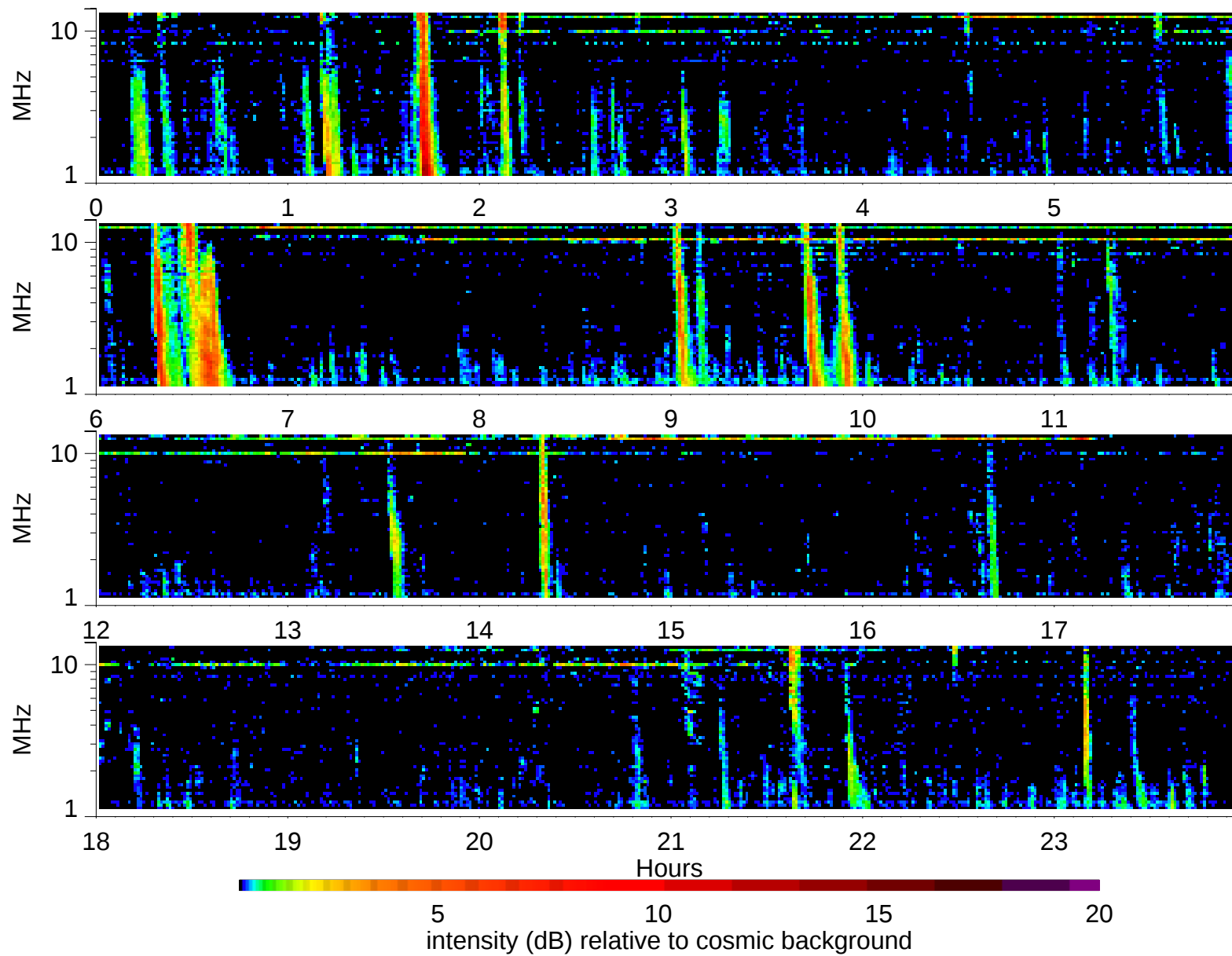
Wind Waves RAD2 receiver: 1999/8/1
