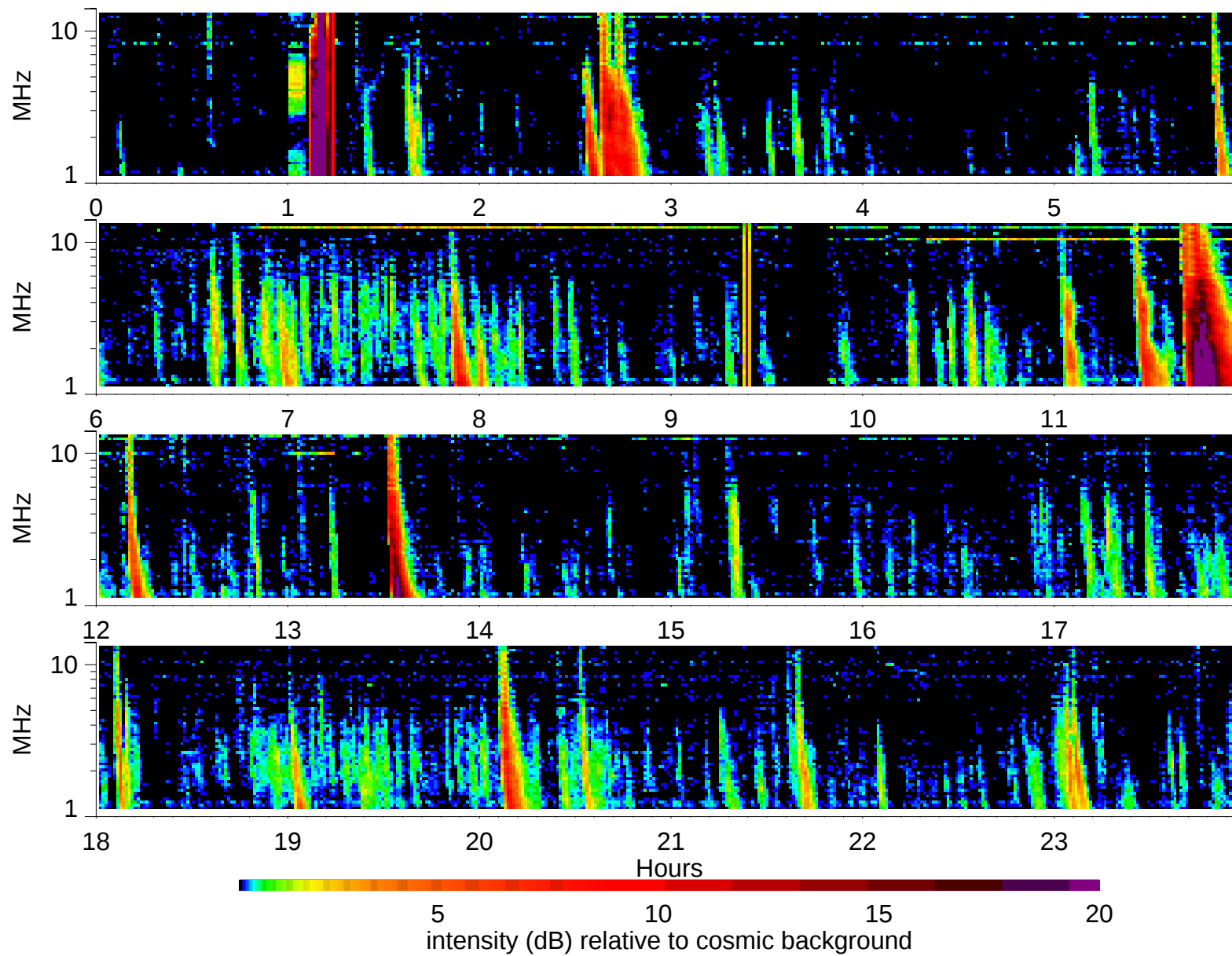
Wind Waves RAD2 receiver: 1999/8/4
