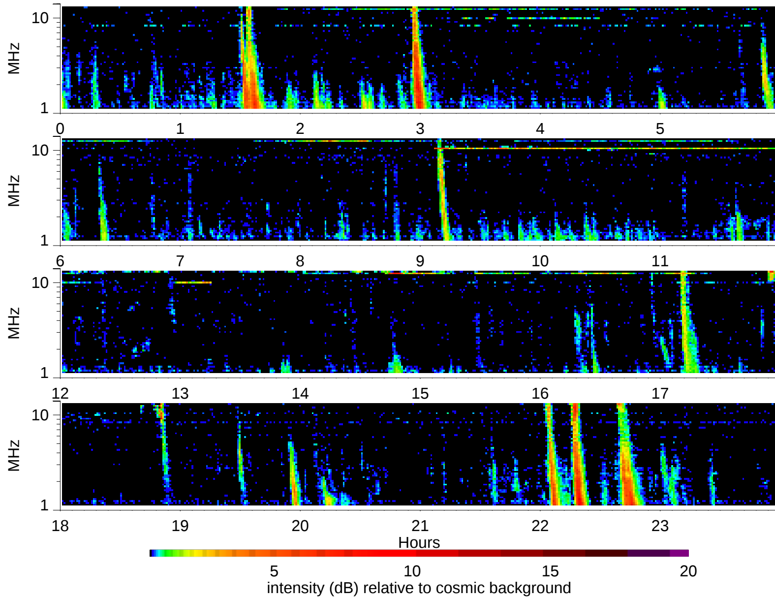
Wind Waves RAD2 receiver: 1999/8/5
