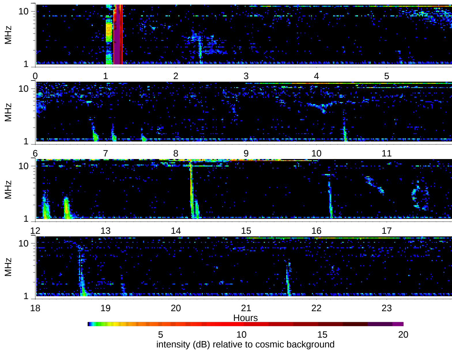
Wind Waves RAD2 receiver: 1999/8/12
