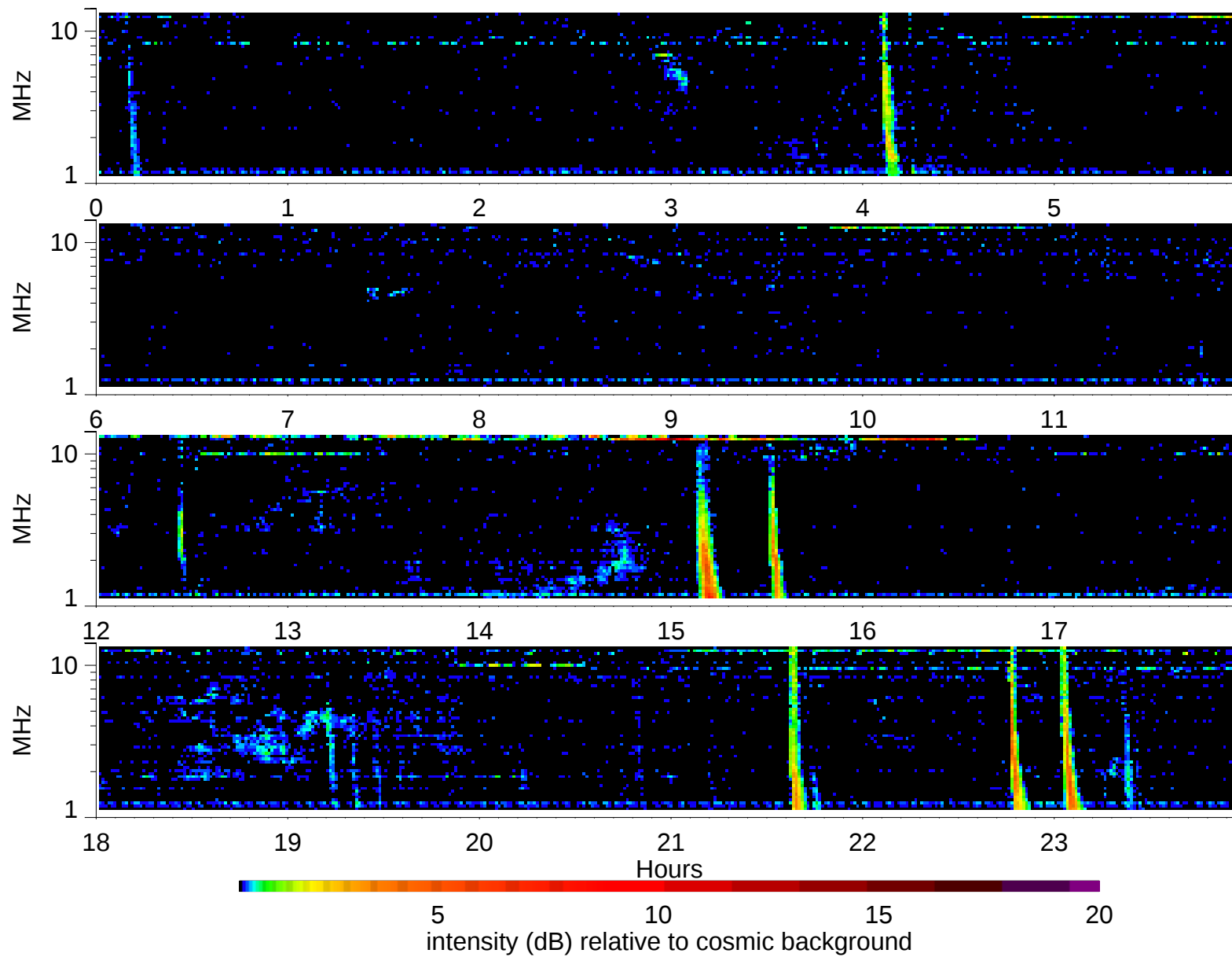
Wind Waves RAD2 receiver: 1999/8/13
