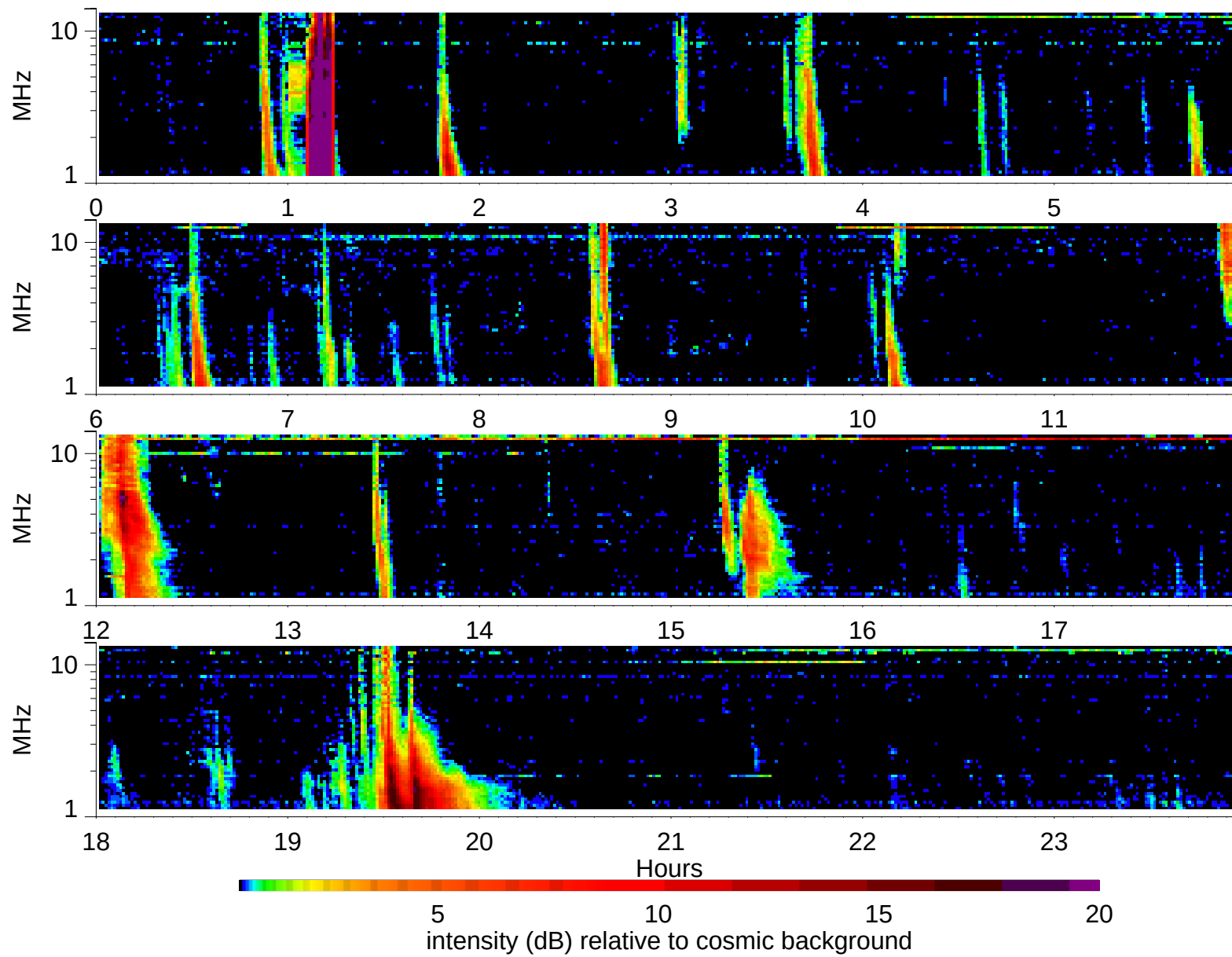
Wind Waves RAD2 receiver: 1999/8/14
