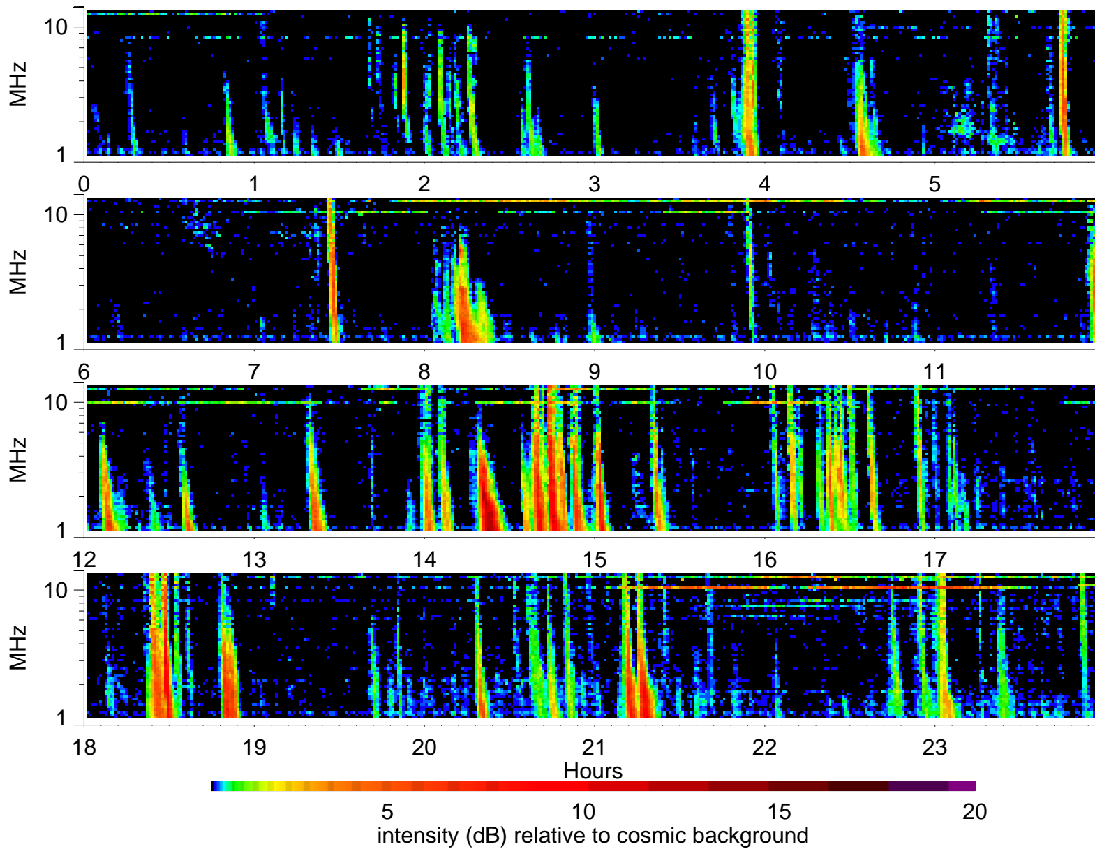
Wind Waves RAD2 receiver: 1999/8/15
