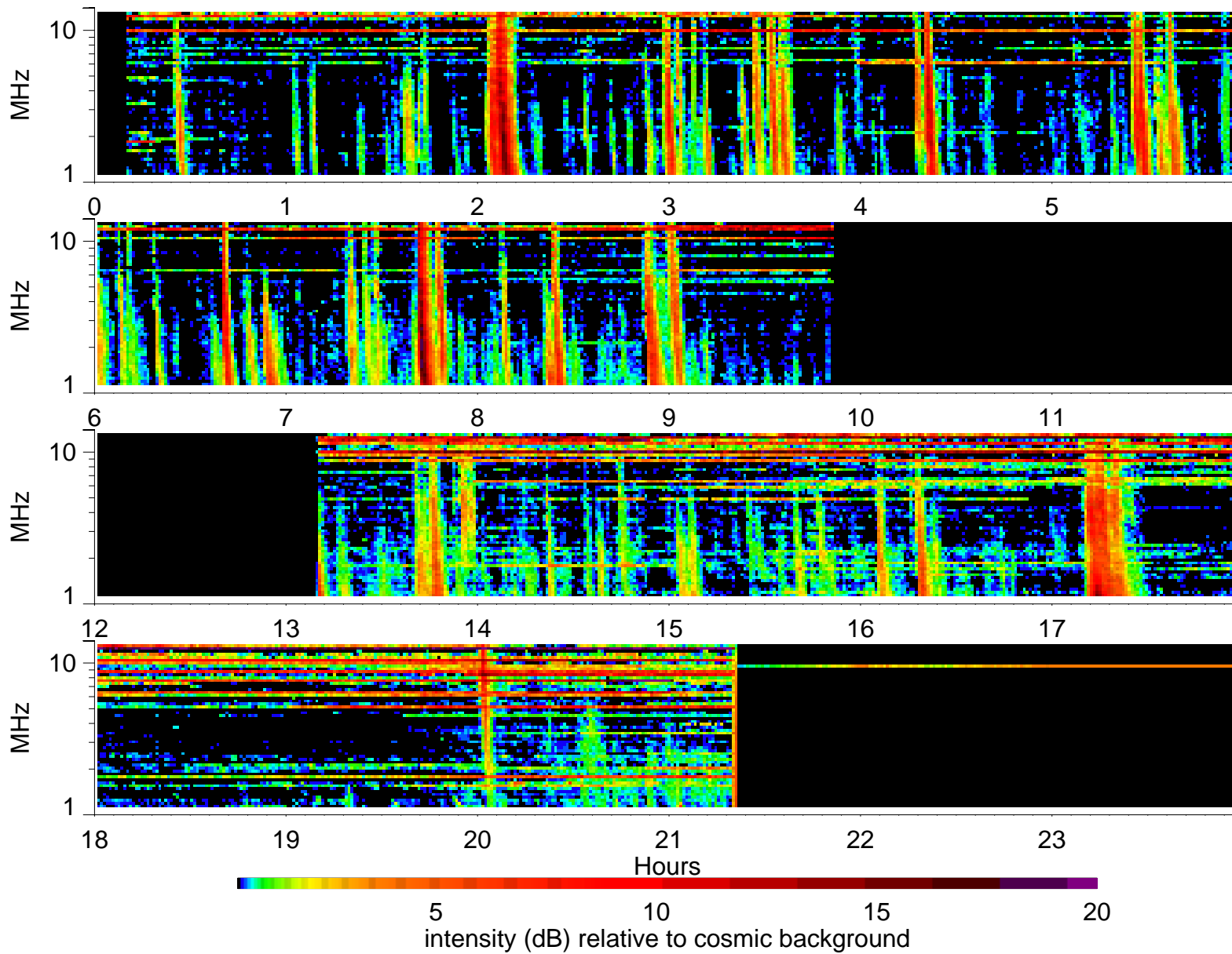
Wind Waves RAD2 receiver: 1999/8/18
