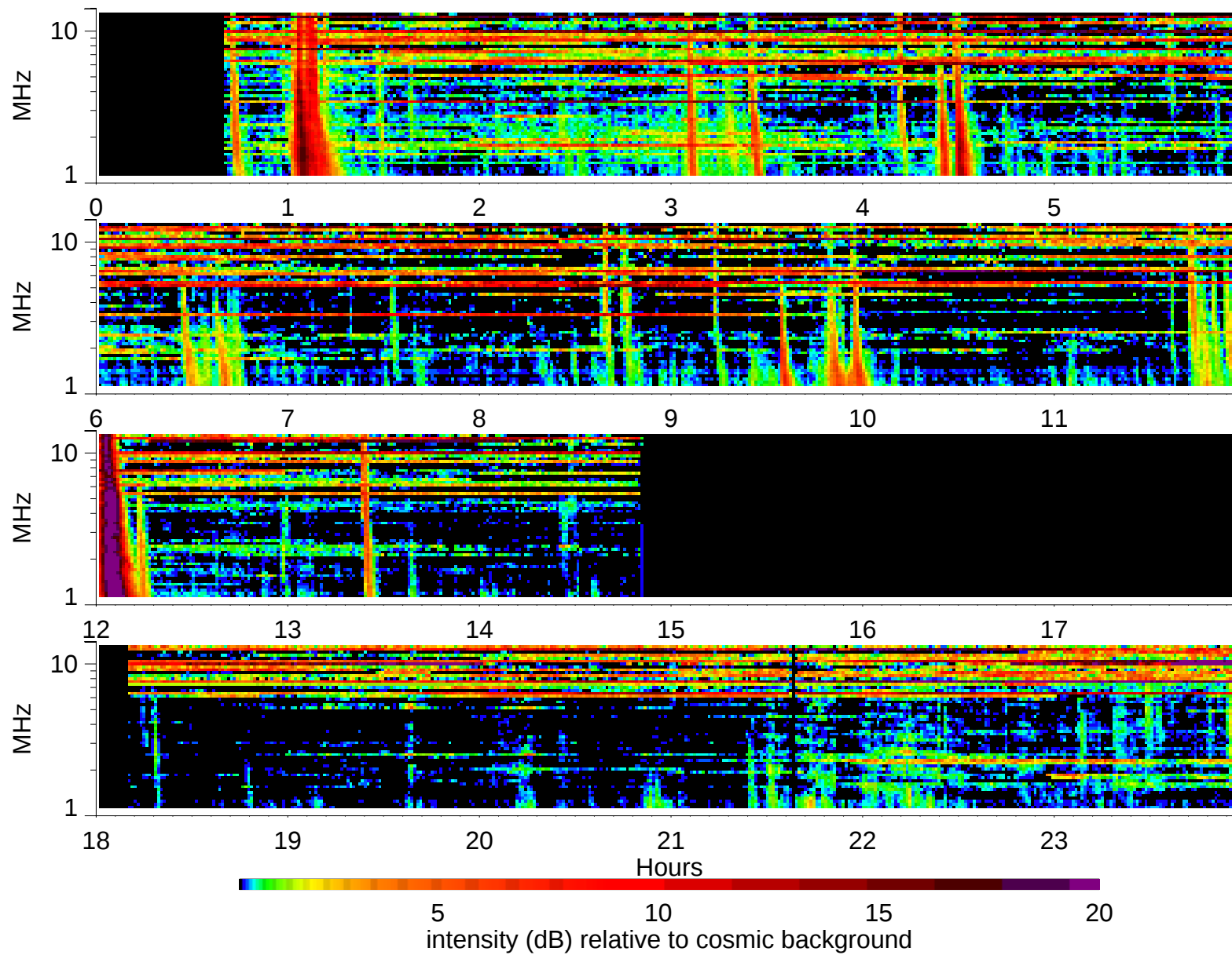
Wind Waves RAD2 receiver: 1999/8/19
