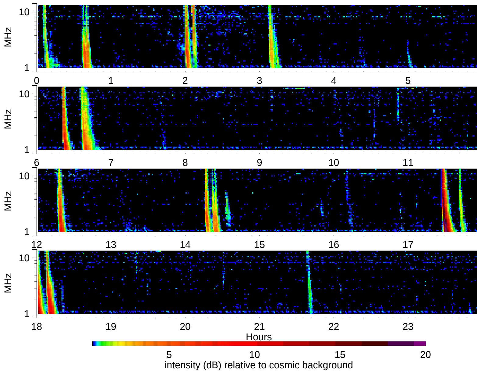
Wind Waves RAD2 receiver: 1999/8/29
