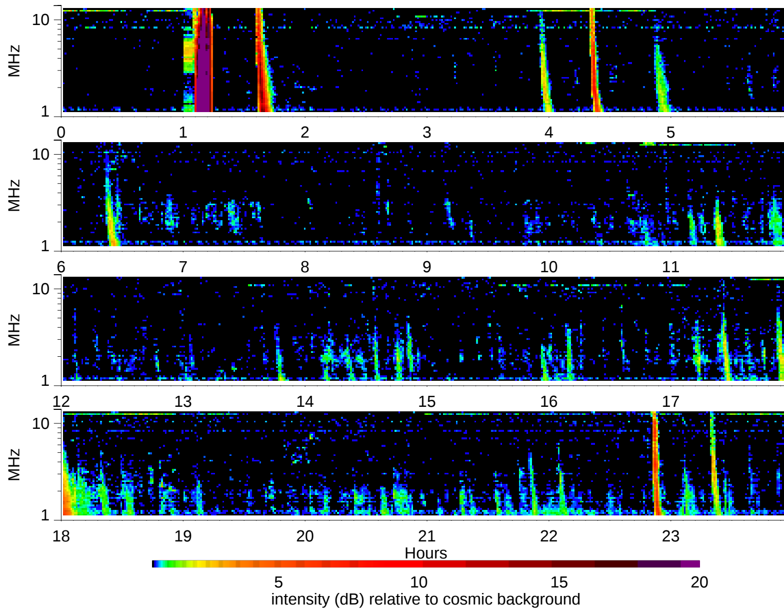
Wind Waves RAD2 receiver: 1999/8/30
