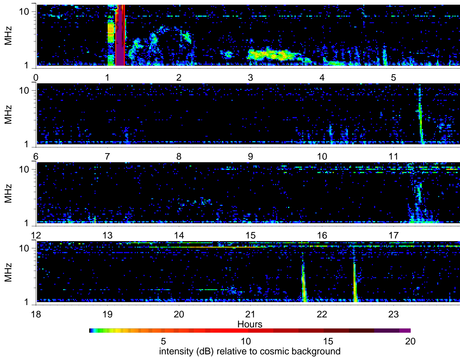
Wind Waves RAD2 receiver: 1999/9/3
