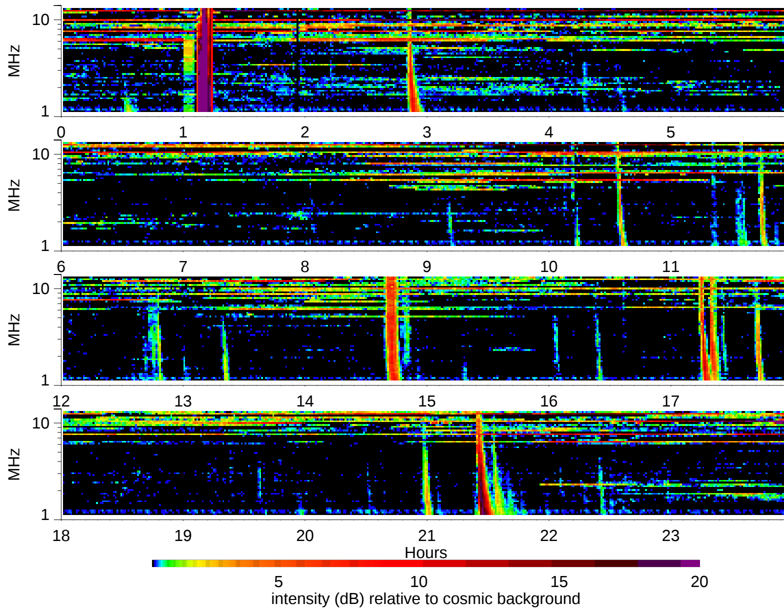
Wind Waves RAD2 receiver: 1999/9/11
