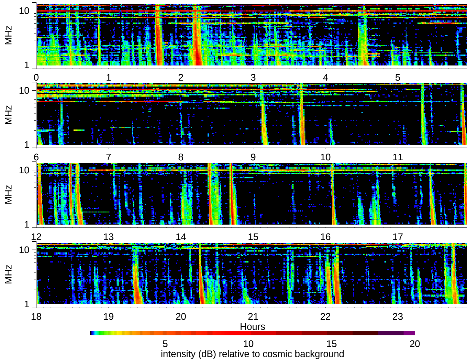
Wind Waves RAD2 receiver: 1999/9/14
