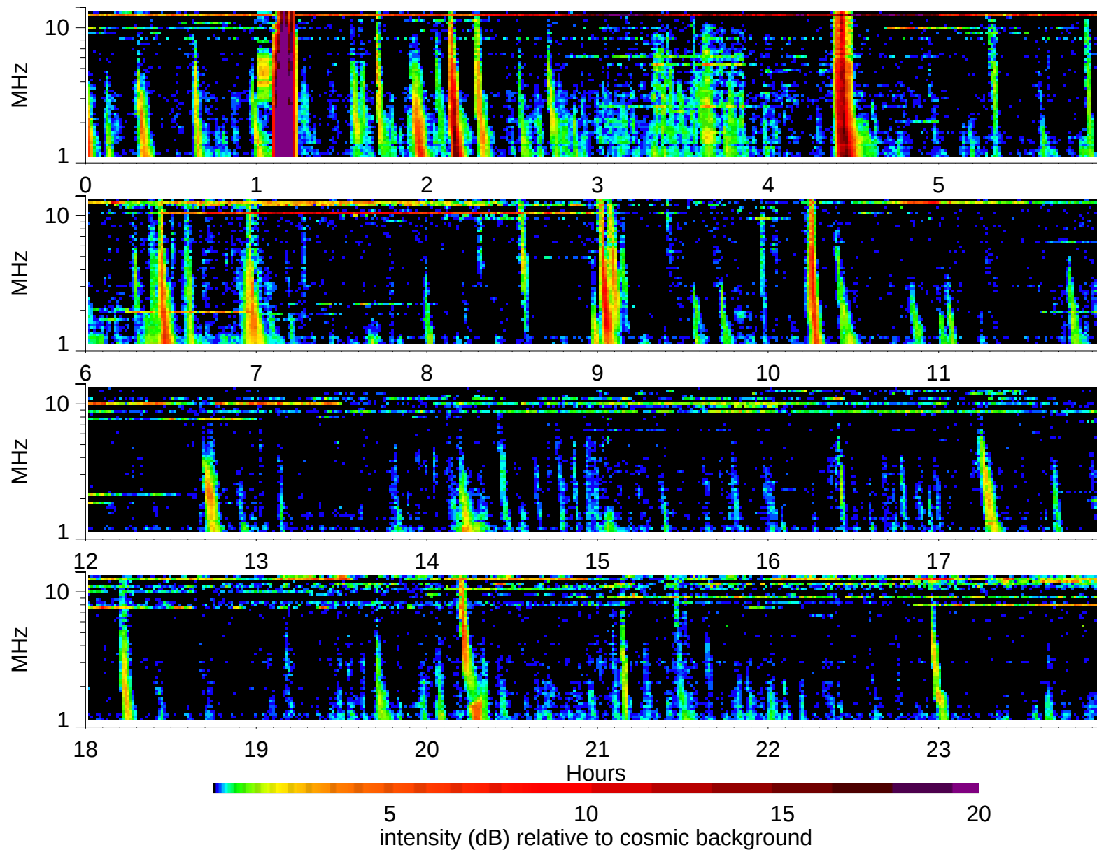
Wind Waves RAD2 receiver: 1999/9/15
