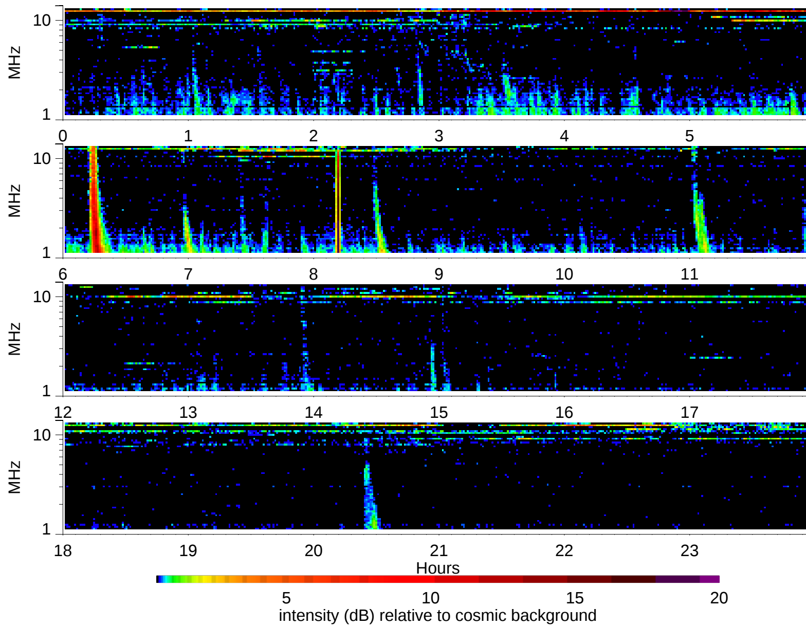
Wind Waves RAD2 receiver: 1999/9/16
