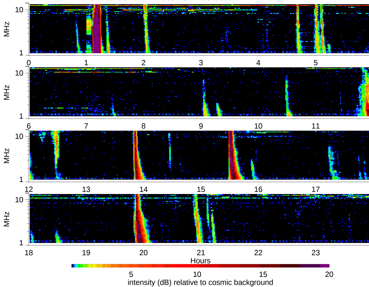
Wind Waves RAD2 receiver: 1999/9/17
