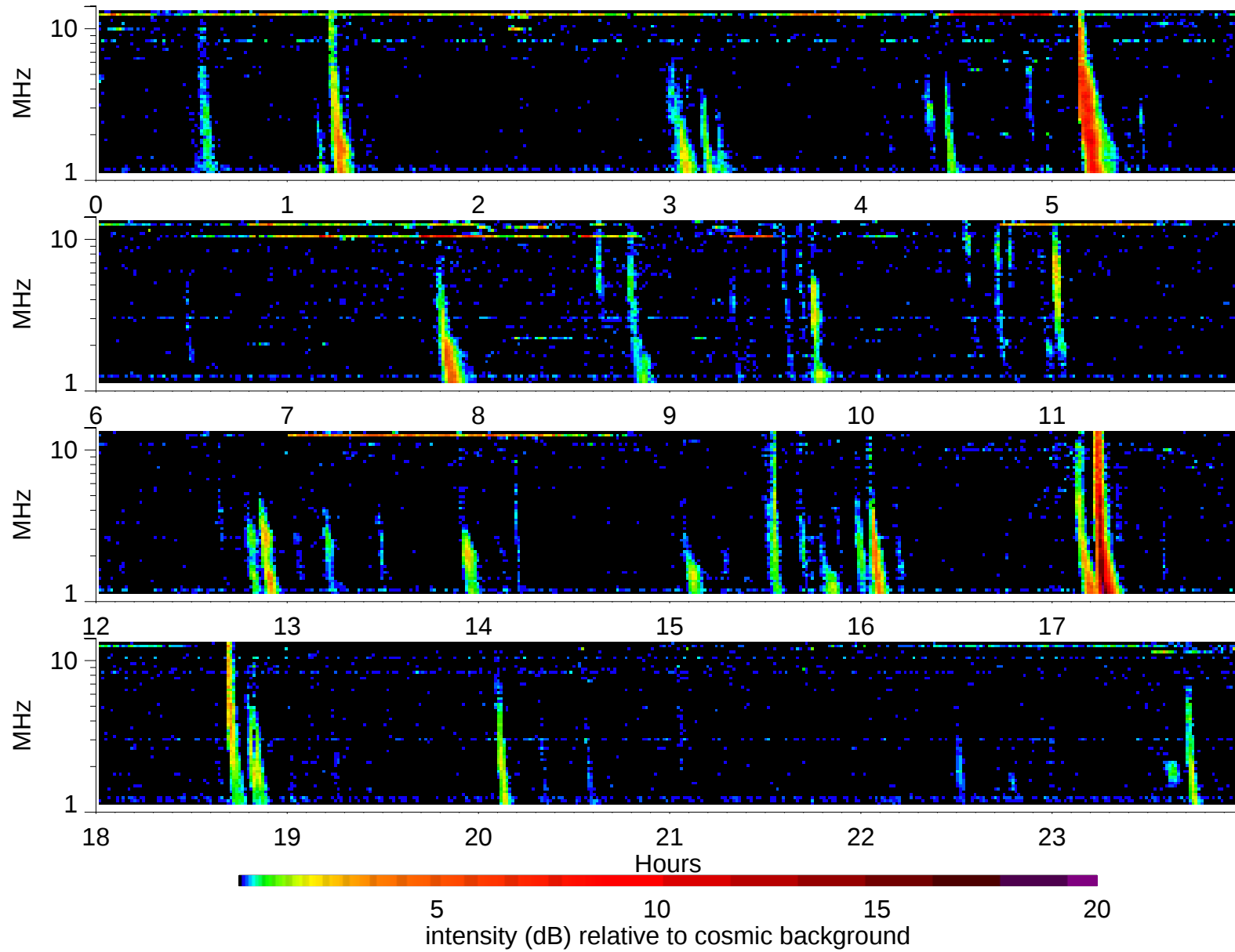
Wind Waves RAD2 receiver: 1999/9/18
