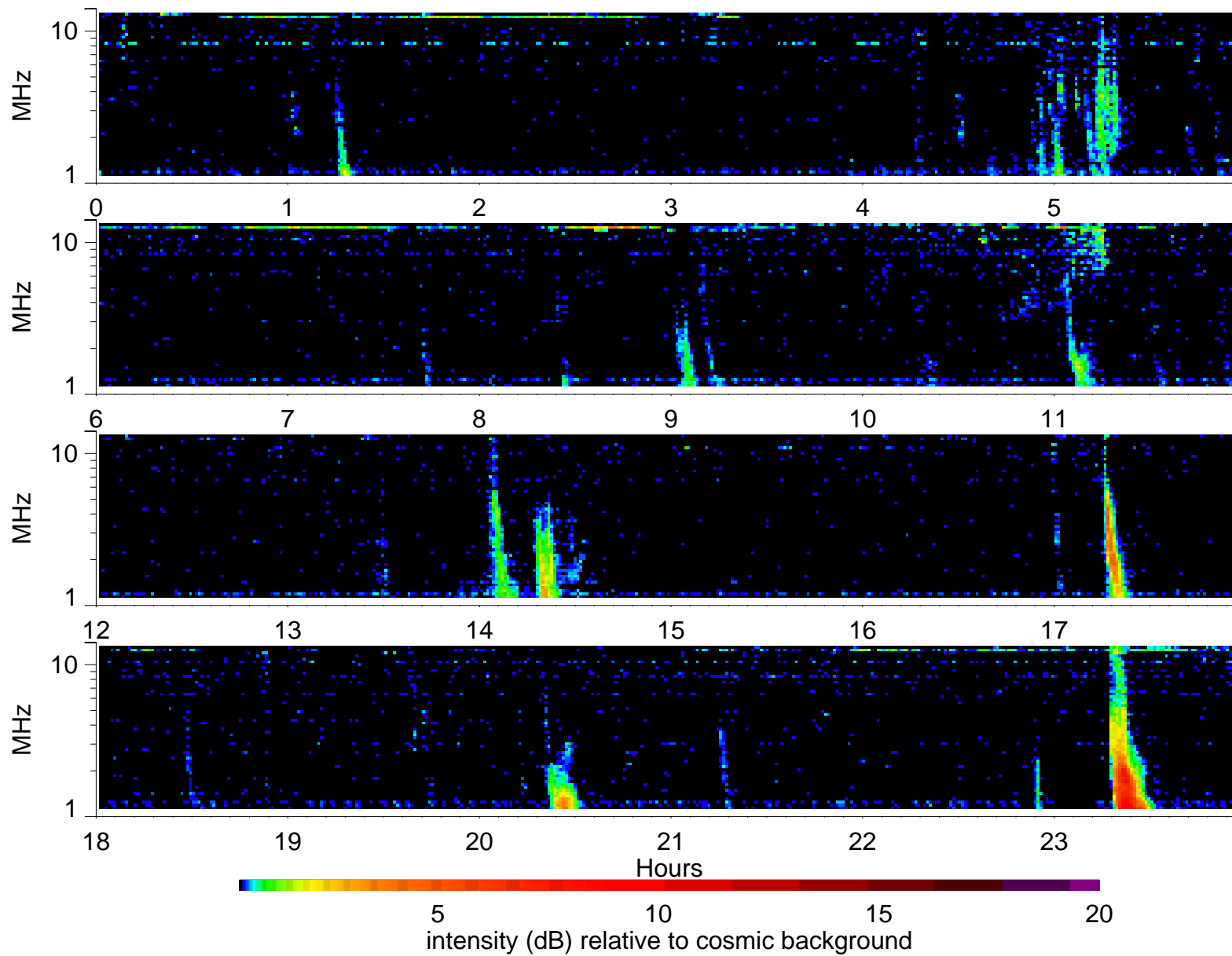
Wind Waves RAD2 receiver: 1999/9/20
