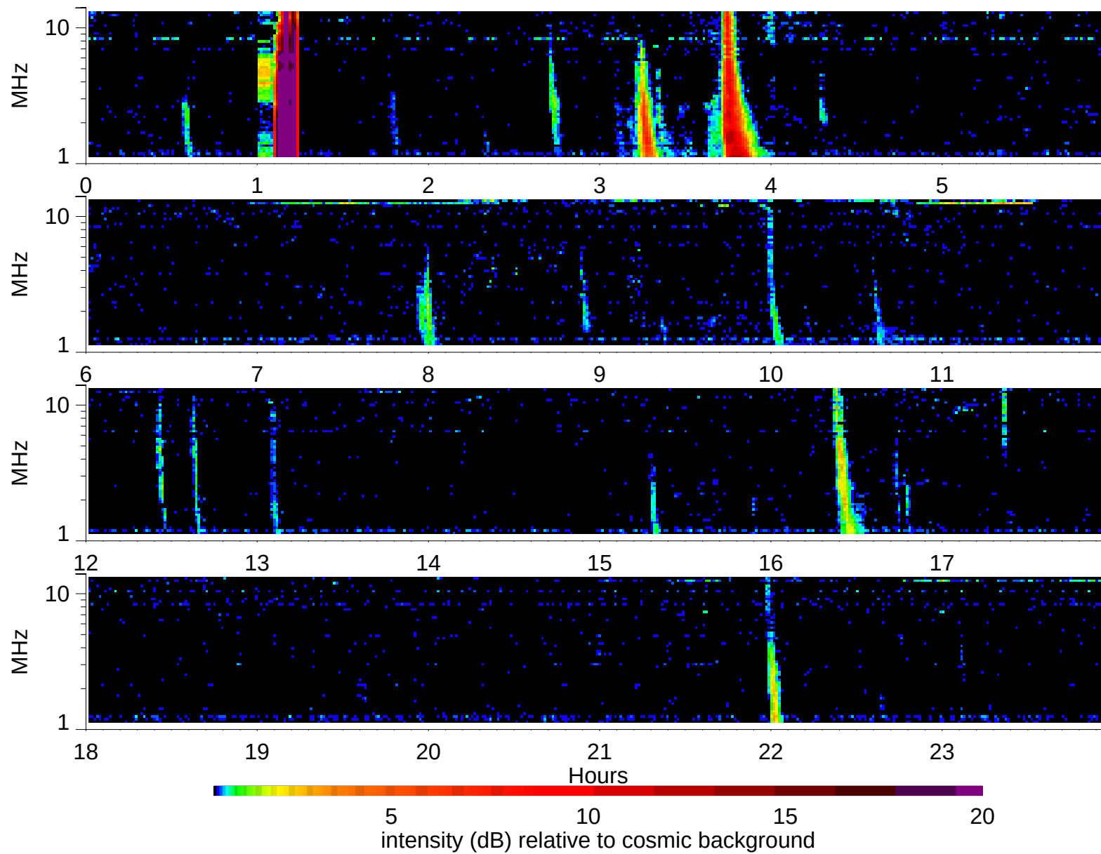
Wind Waves RAD2 receiver: 1999/9/21
