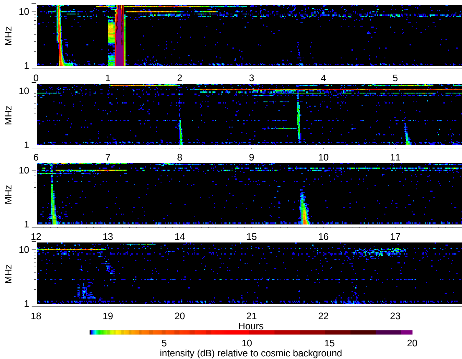
Wind Waves RAD2 receiver: 1999/9/23
