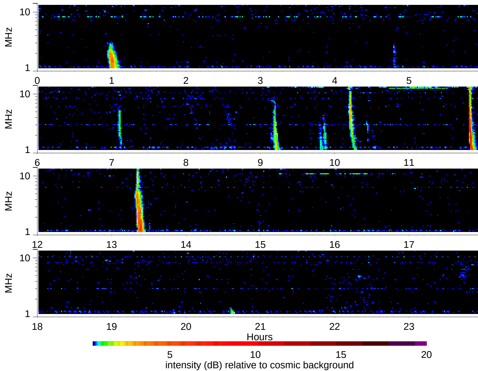
Wind Waves RAD2 receiver: 1999/9/24
