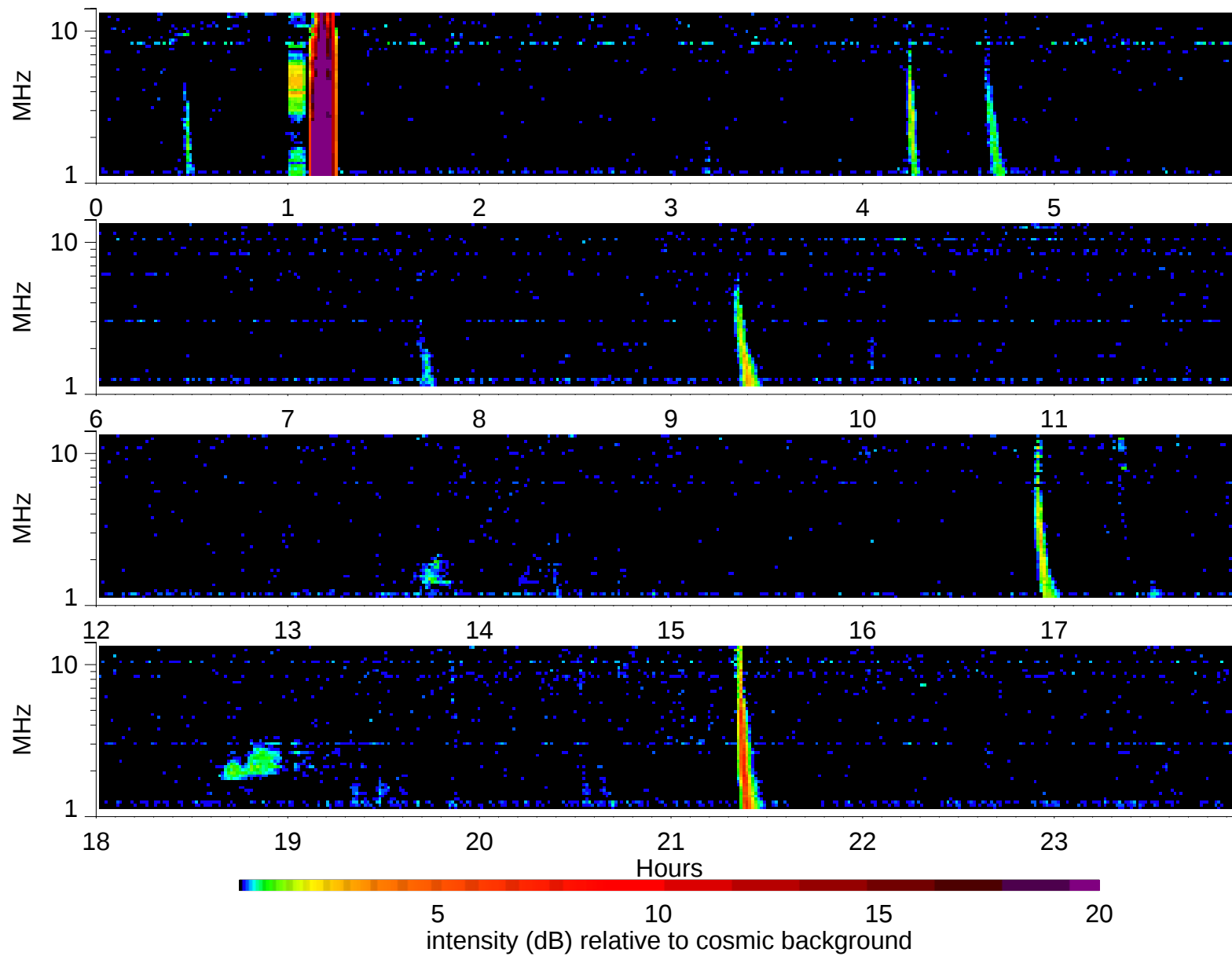
Wind Waves RAD2 receiver: 1999/9/25
