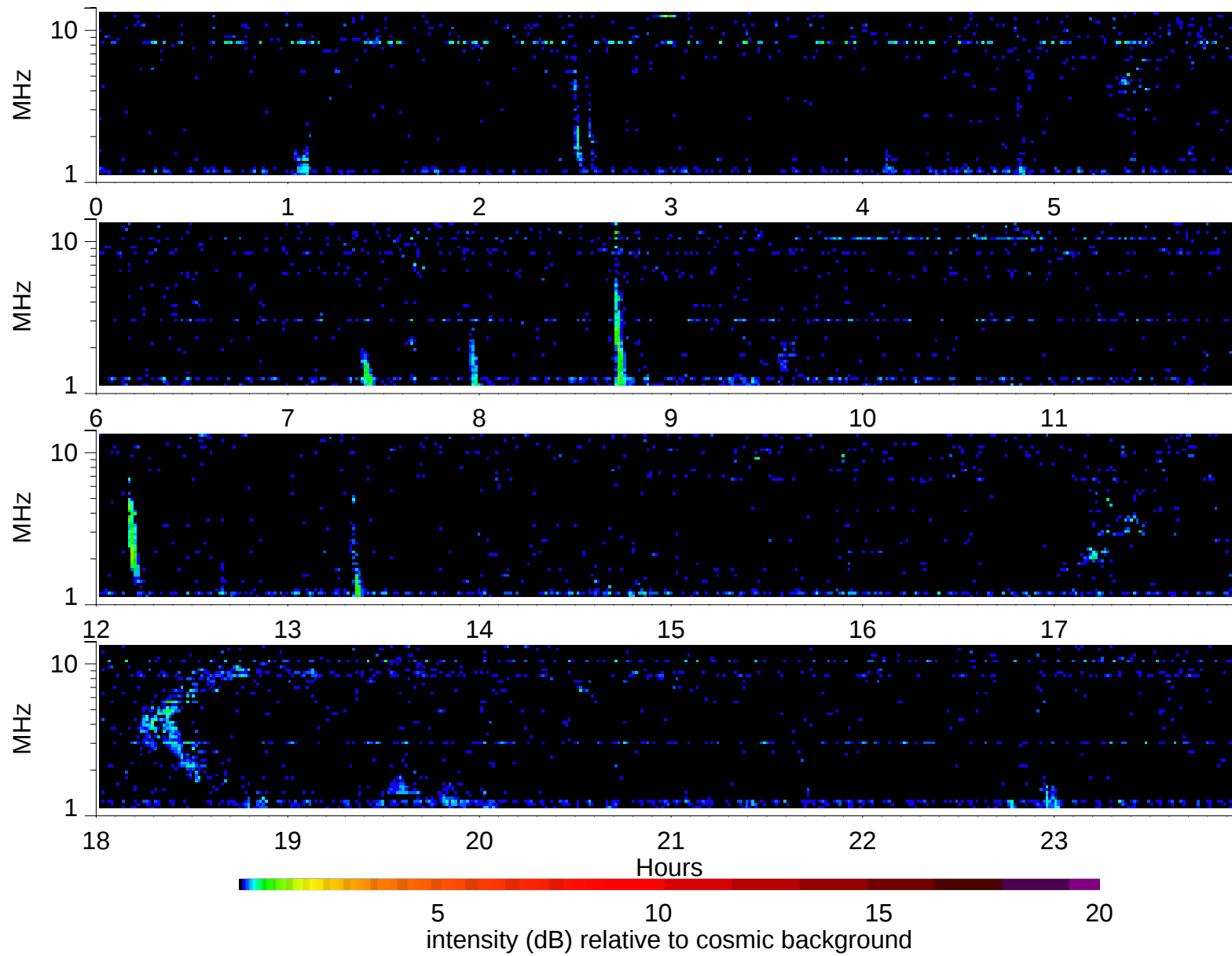
Wind Waves RAD2 receiver: 1999/9/26
