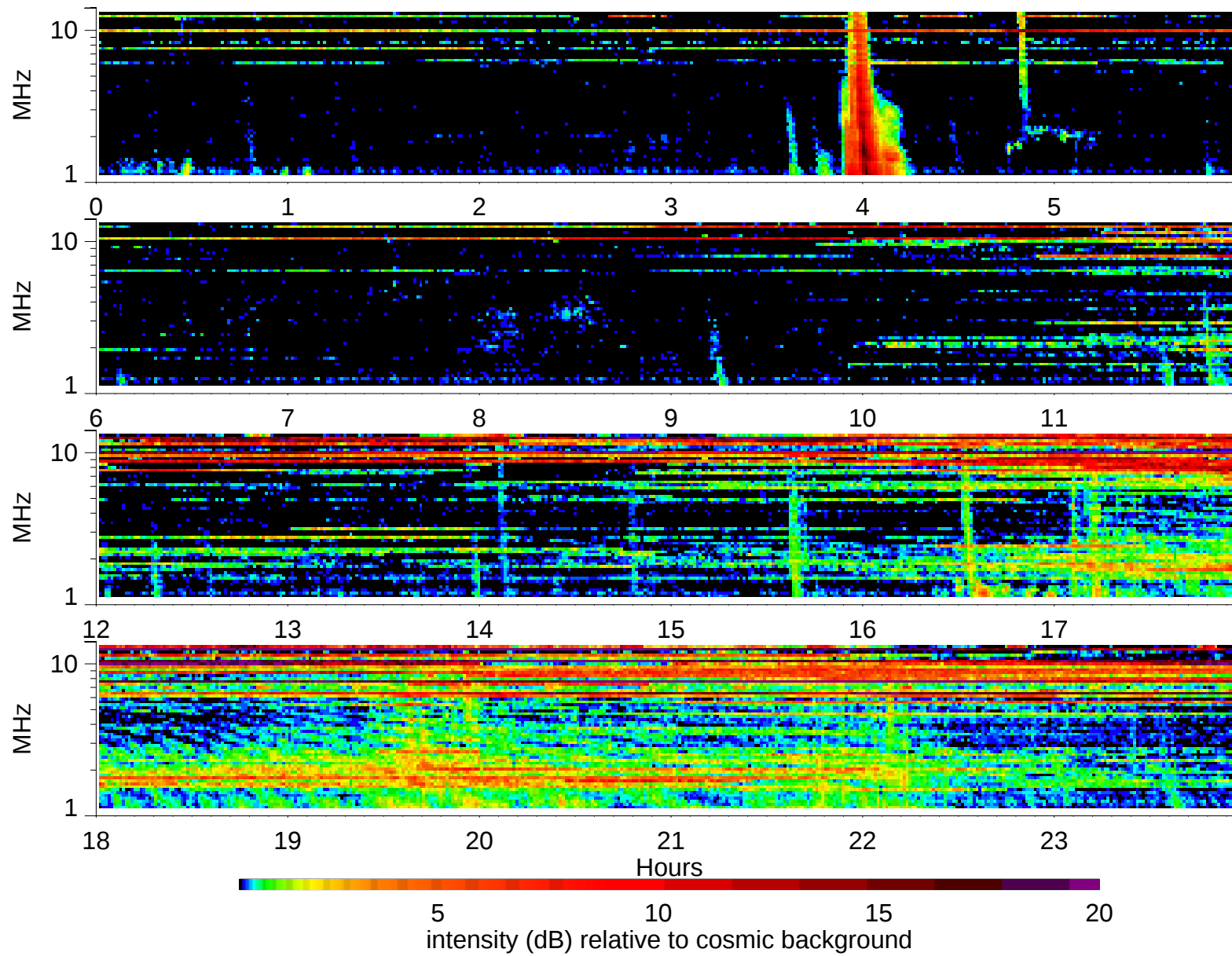
Wind Waves RAD2 receiver: 1999/9/30
