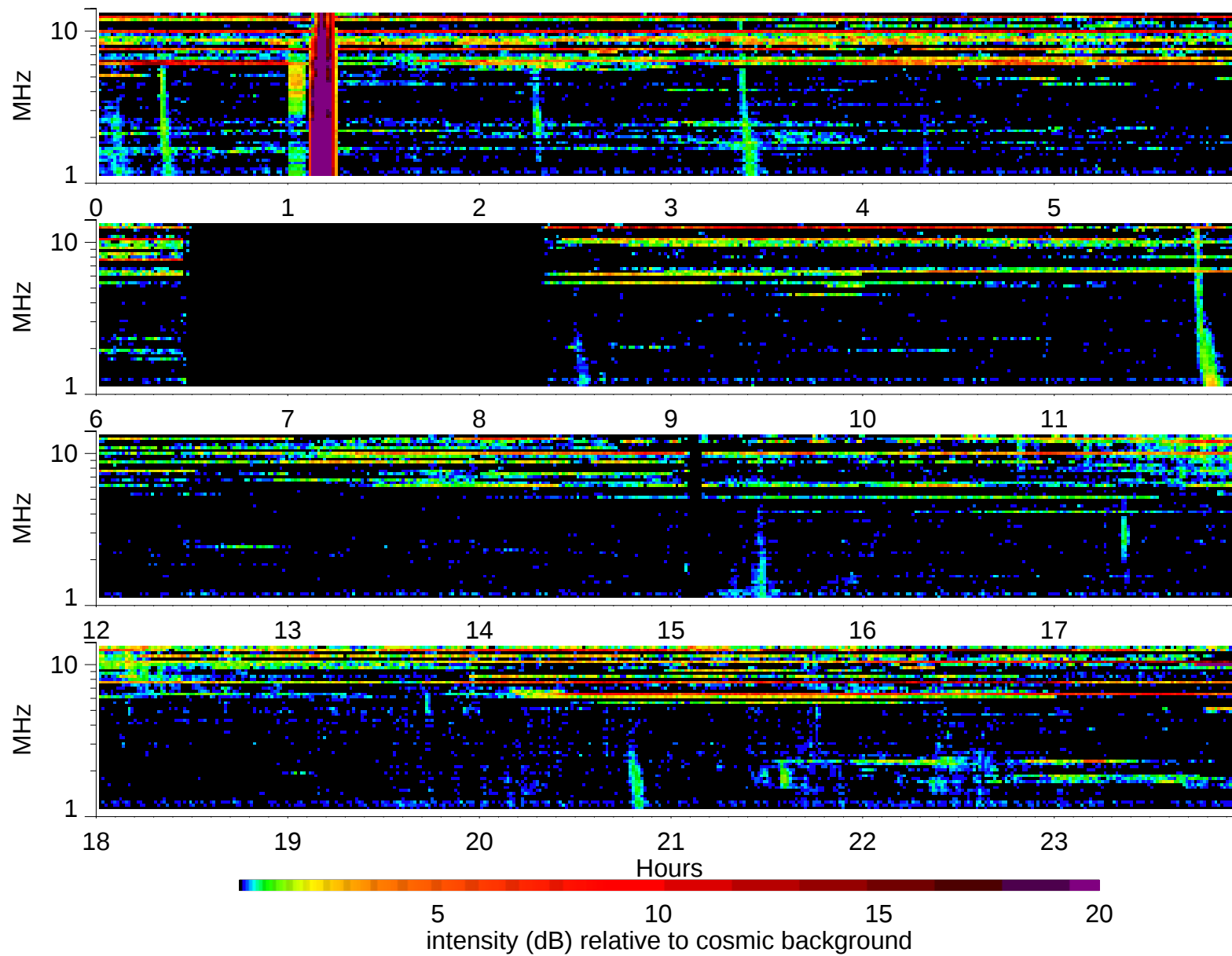
Wind Waves RAD2 receiver: 1999/10/3
