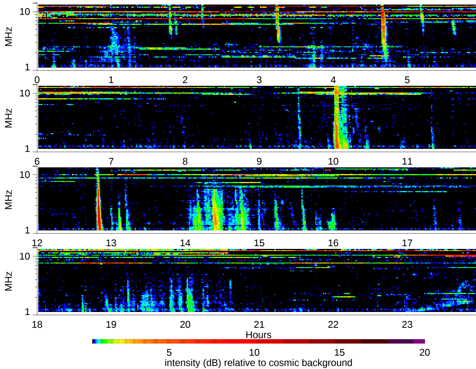
Wind Waves RAD2 receiver: 1999/10/8
