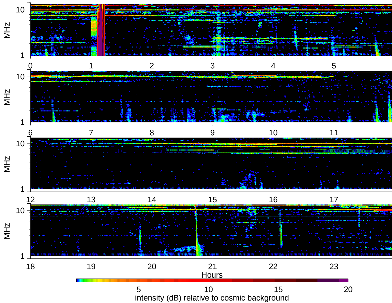
Wind Waves RAD2 receiver: 1999/10/9
