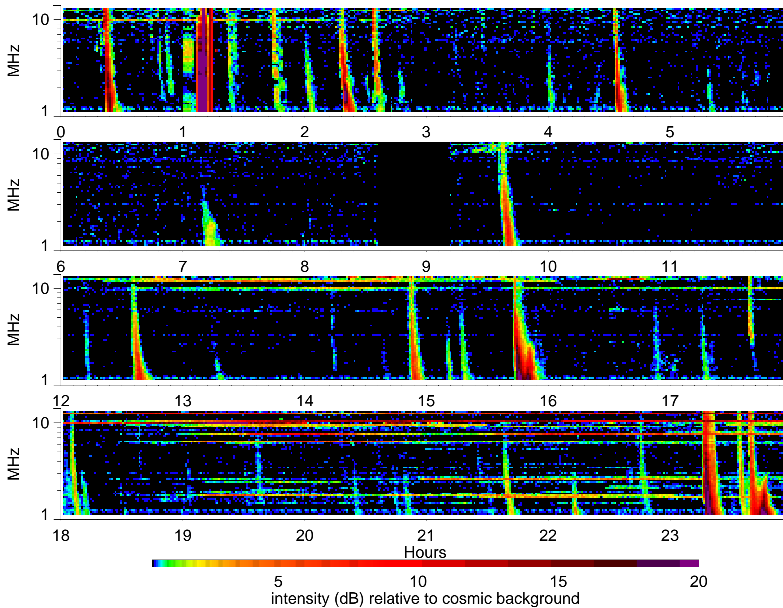
Wind Waves RAD2 receiver: 1999/10/13
