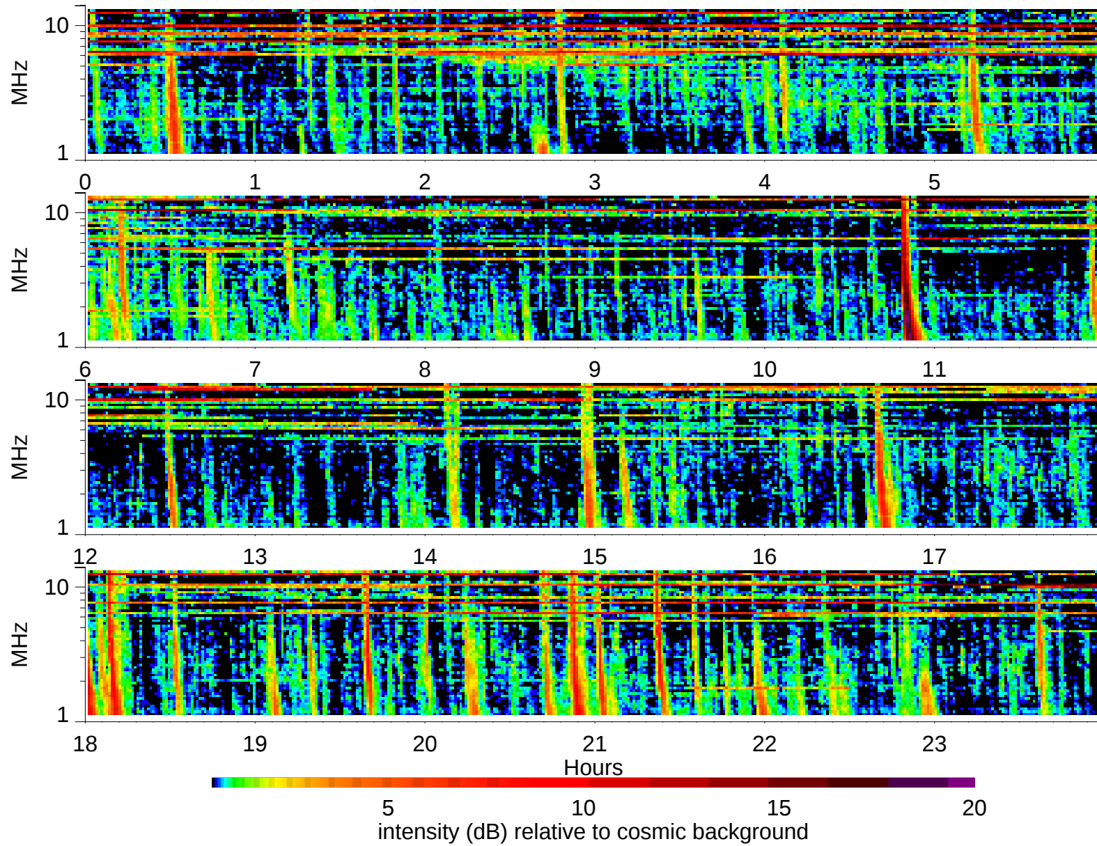
Wind Waves RAD2 receiver: 1999/10/16
