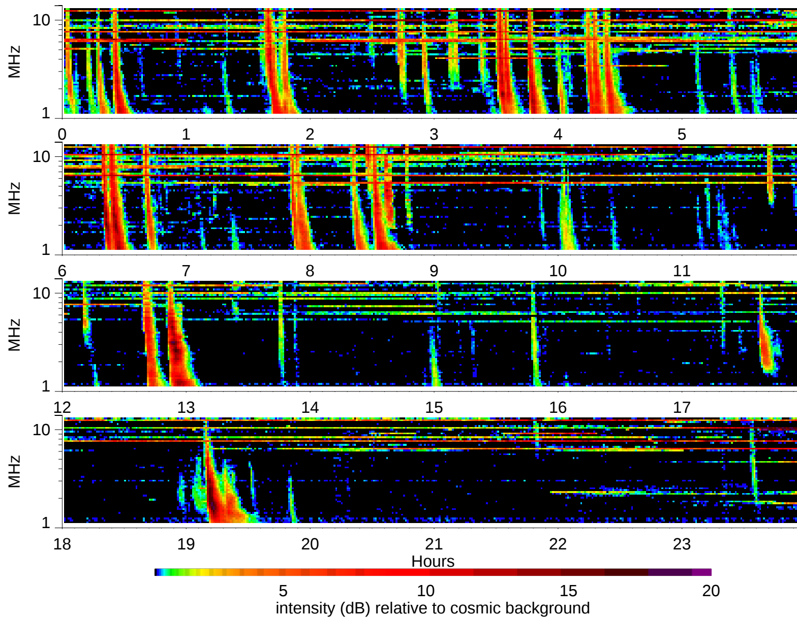
Wind Waves RAD2 receiver: 1999/10/22
