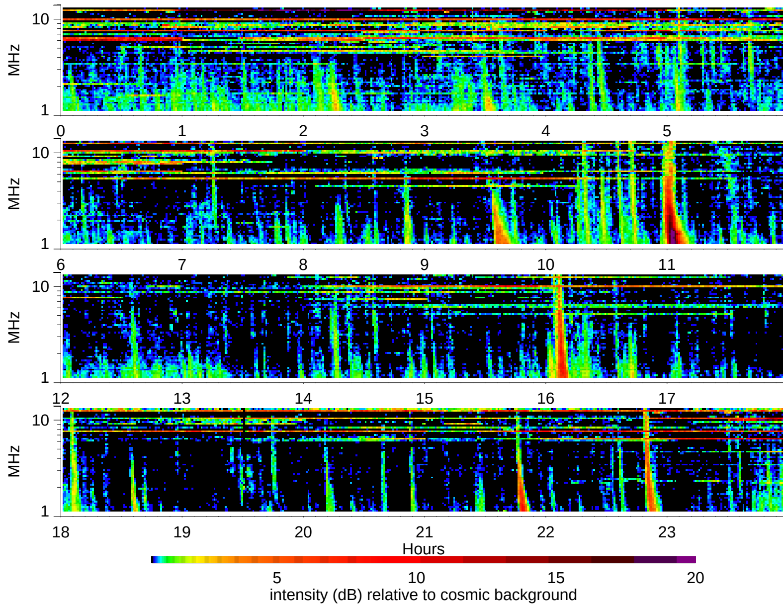
Wind Waves RAD2 receiver: 1999/10/24
