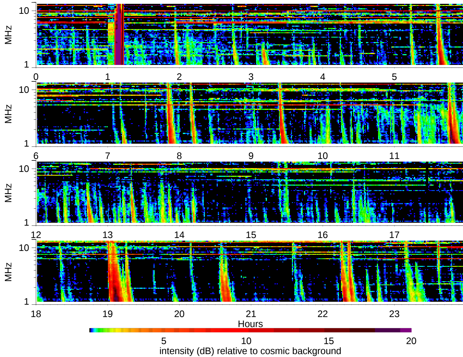
Wind Waves RAD2 receiver: 1999/10/25
