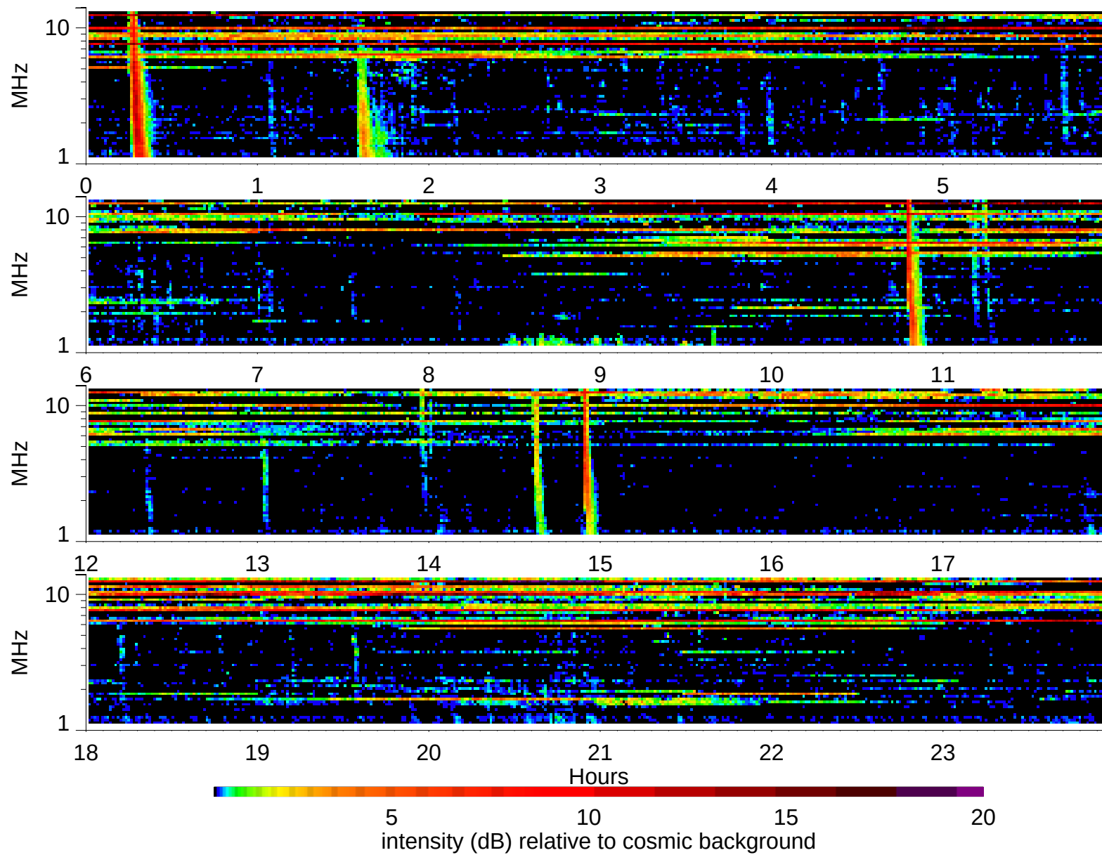
Wind Waves RAD2 receiver: 1999/11/1
