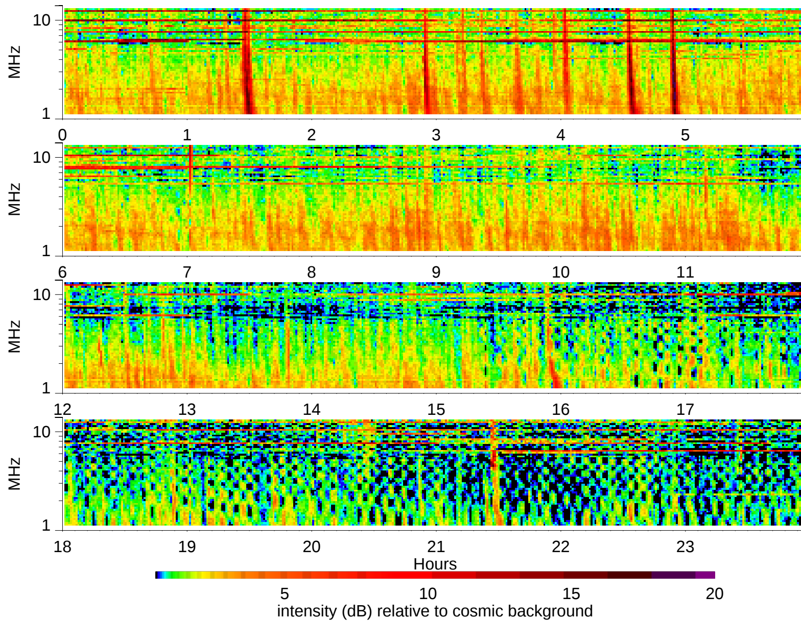
Wind Waves RAD2 receiver: 1999/11/11
