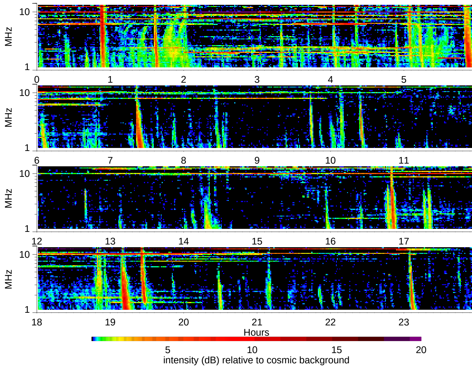
Wind Waves RAD2 receiver: 1999/11/13
