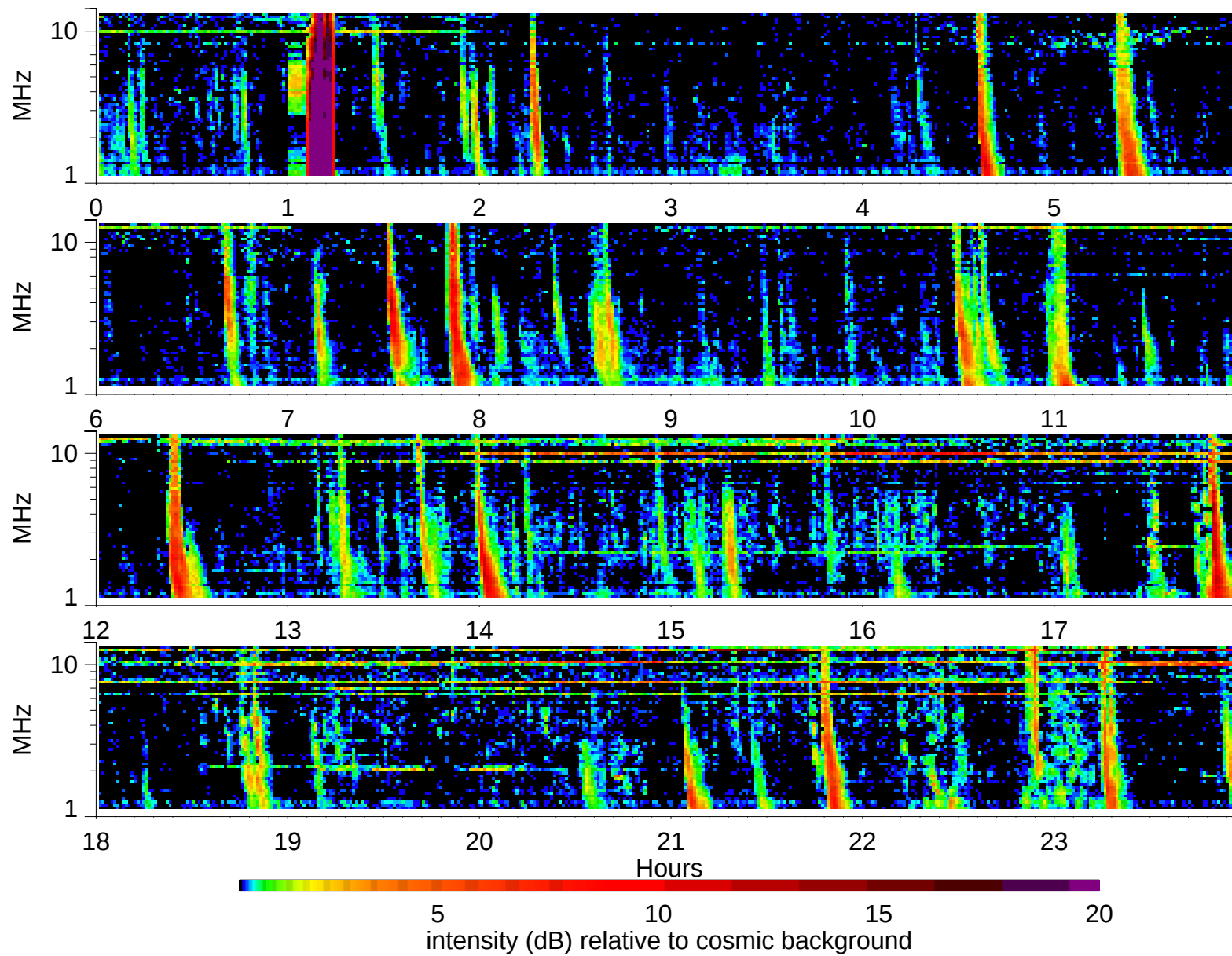
Wind Waves RAD2 receiver: 1999/11/14
