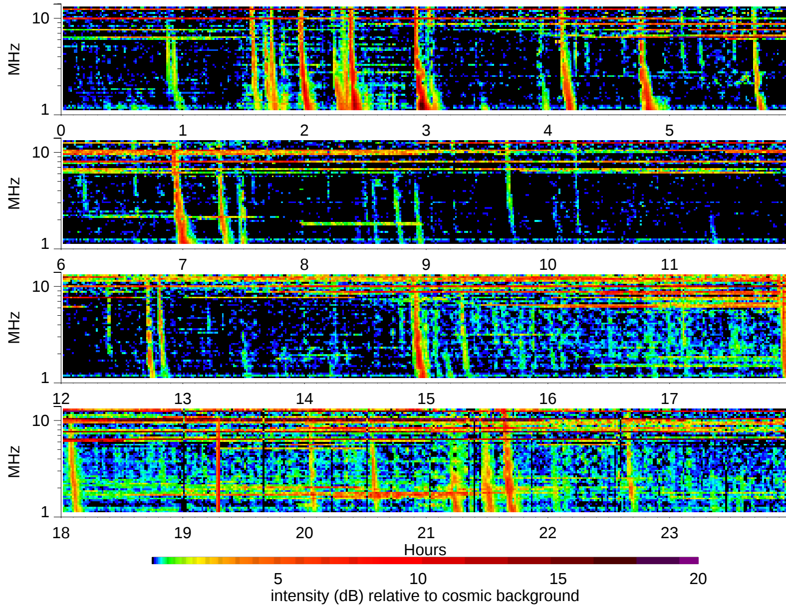
Wind Waves RAD2 receiver: 1999/11/15
