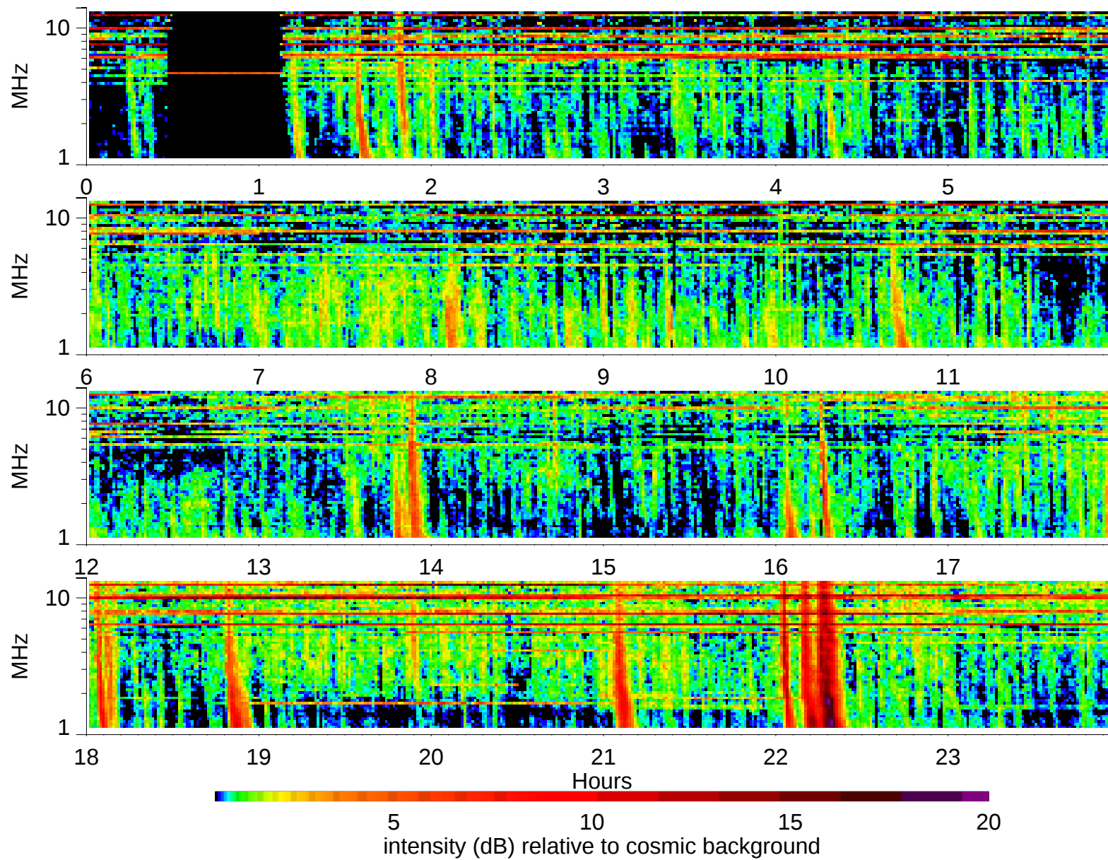
Wind Waves RAD2 receiver: 1999/11/18
