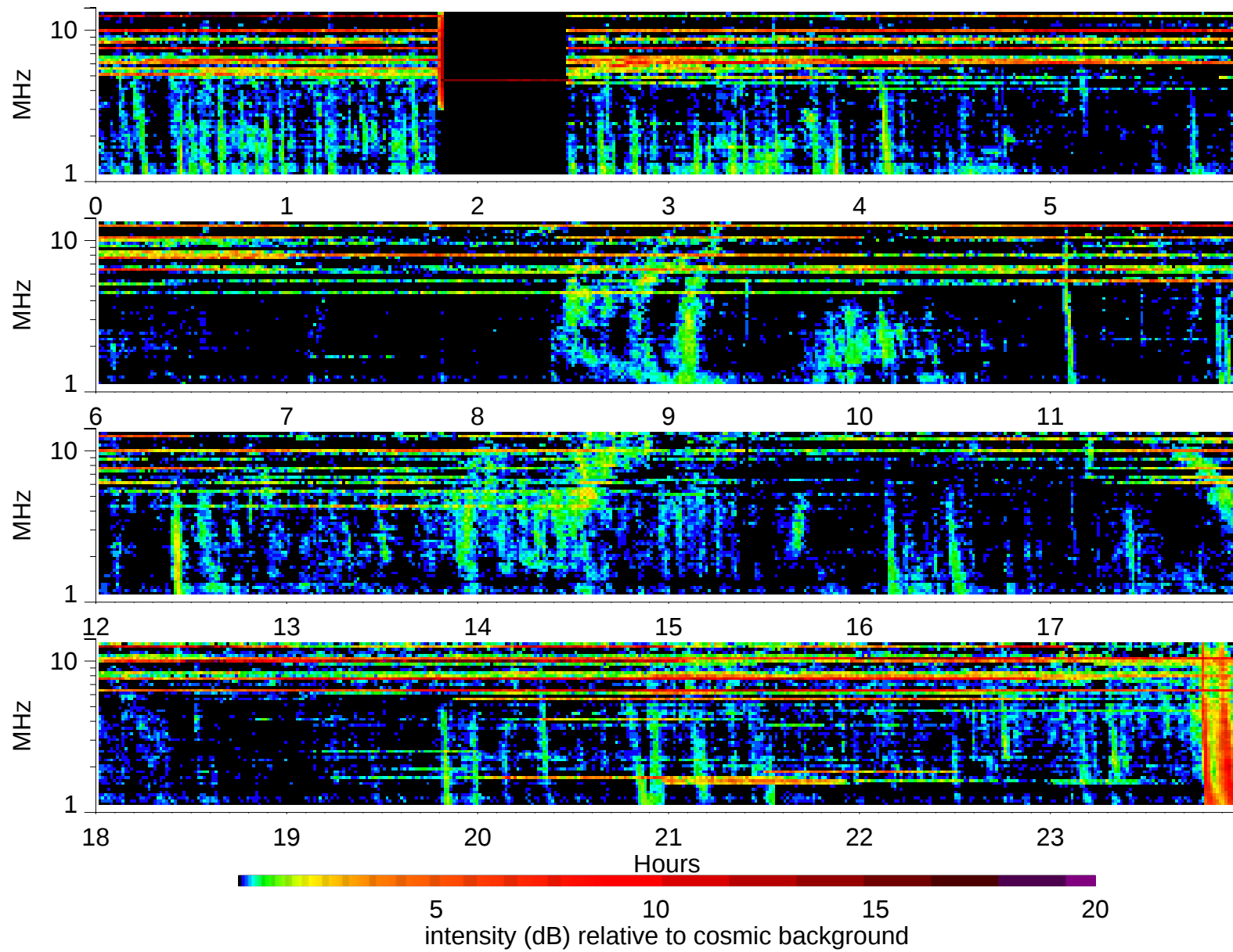
Wind Waves RAD2 receiver: 1999/11/21
