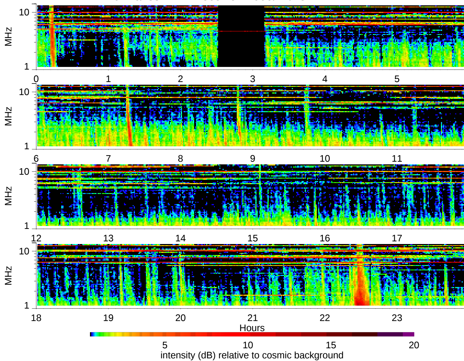
Wind Waves RAD2 receiver: 1999/11/23
