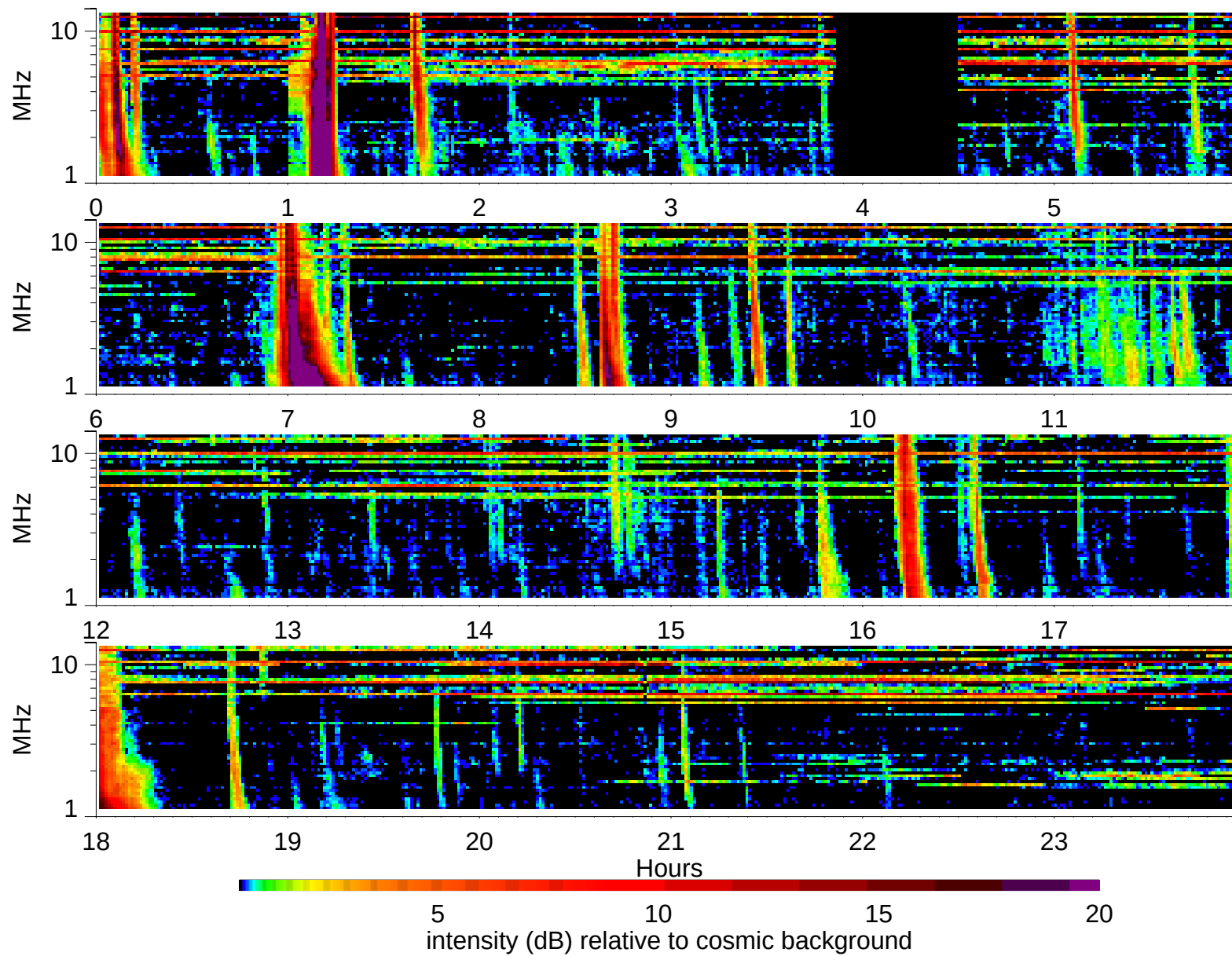
Wind Waves RAD2 receiver: 1999/11/26
