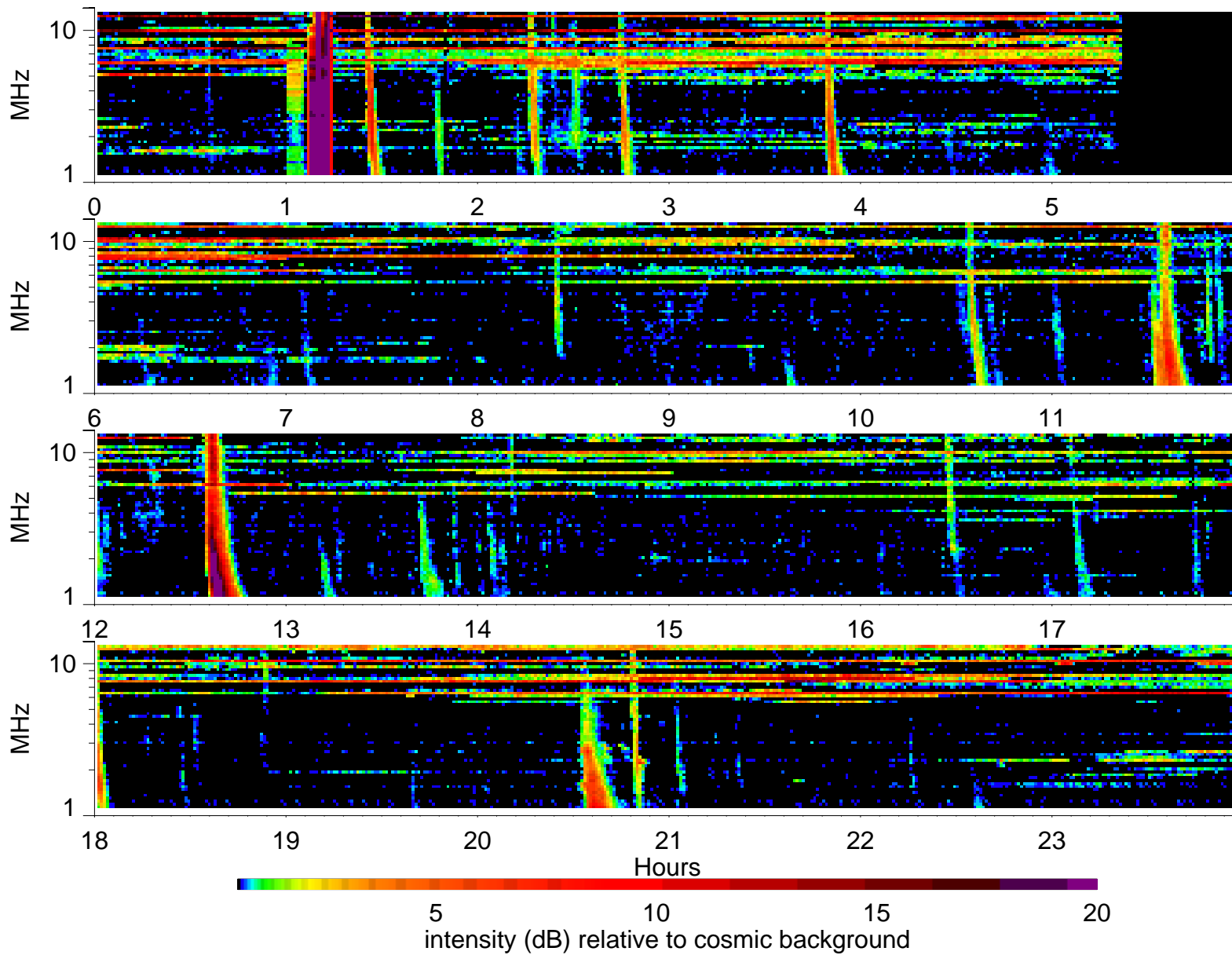
Wind Waves RAD2 receiver: 1999/11/28
