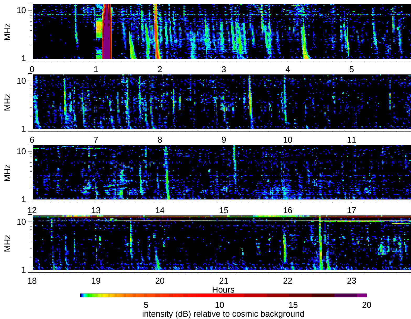
Wind Waves RAD2 receiver: 1999/11/30
