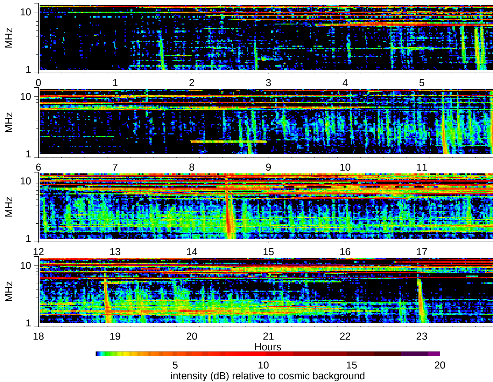
Wind Waves RAD2 receiver: 1999/12/1
