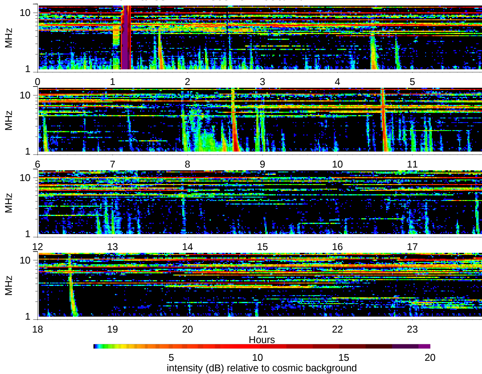
Wind Waves RAD2 receiver: 1999/12/12
