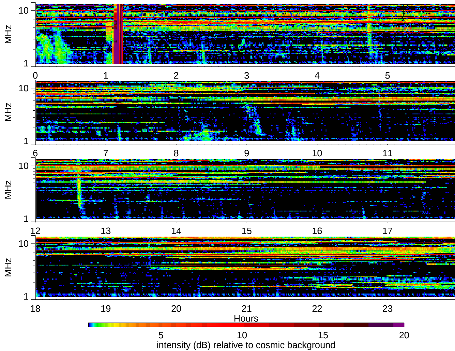
Wind Waves RAD2 receiver: 1999/12/14
