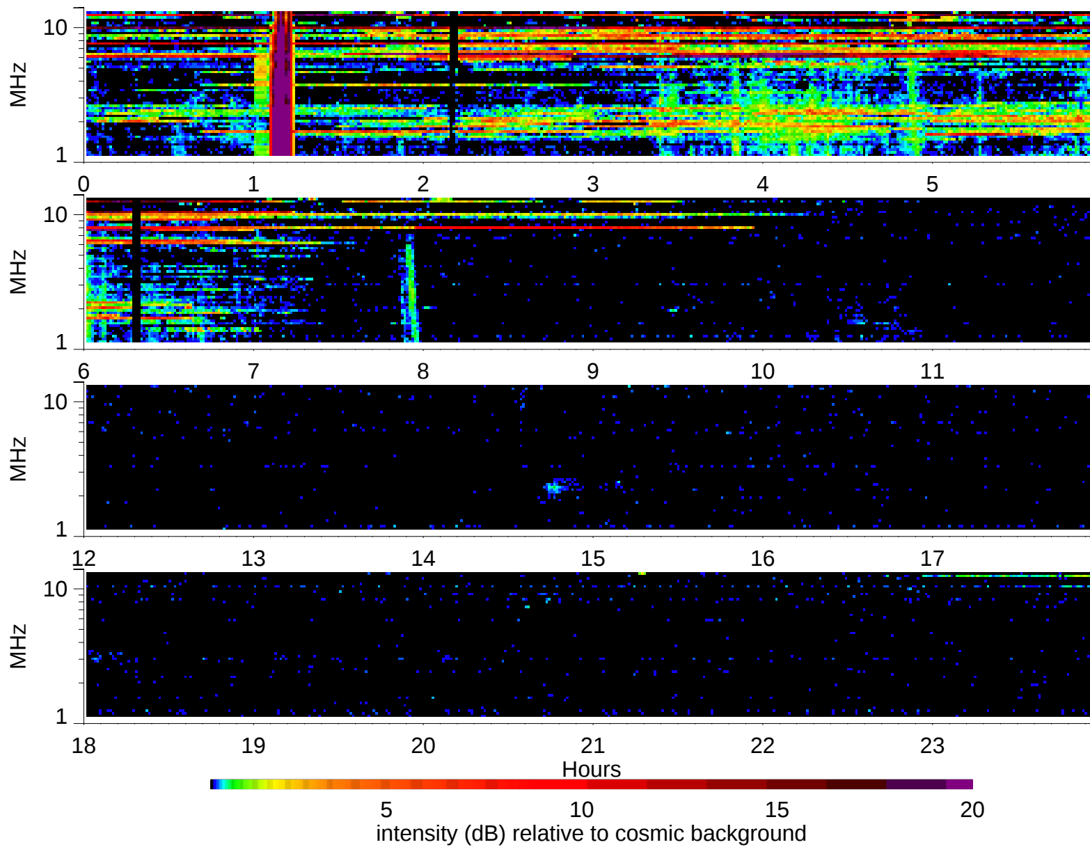
Wind Waves RAD2 receiver: 1999/12/16
