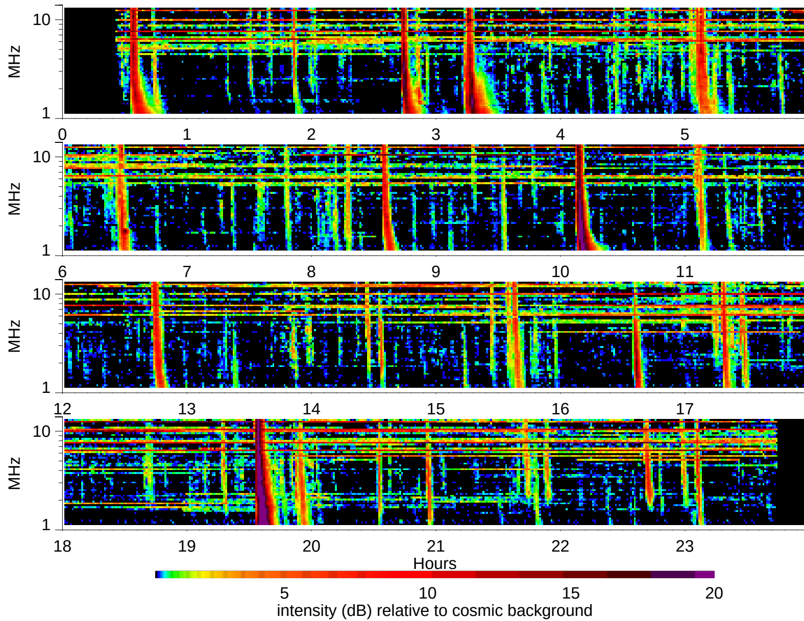
Wind Waves RAD2 receiver: 1999/12/23
