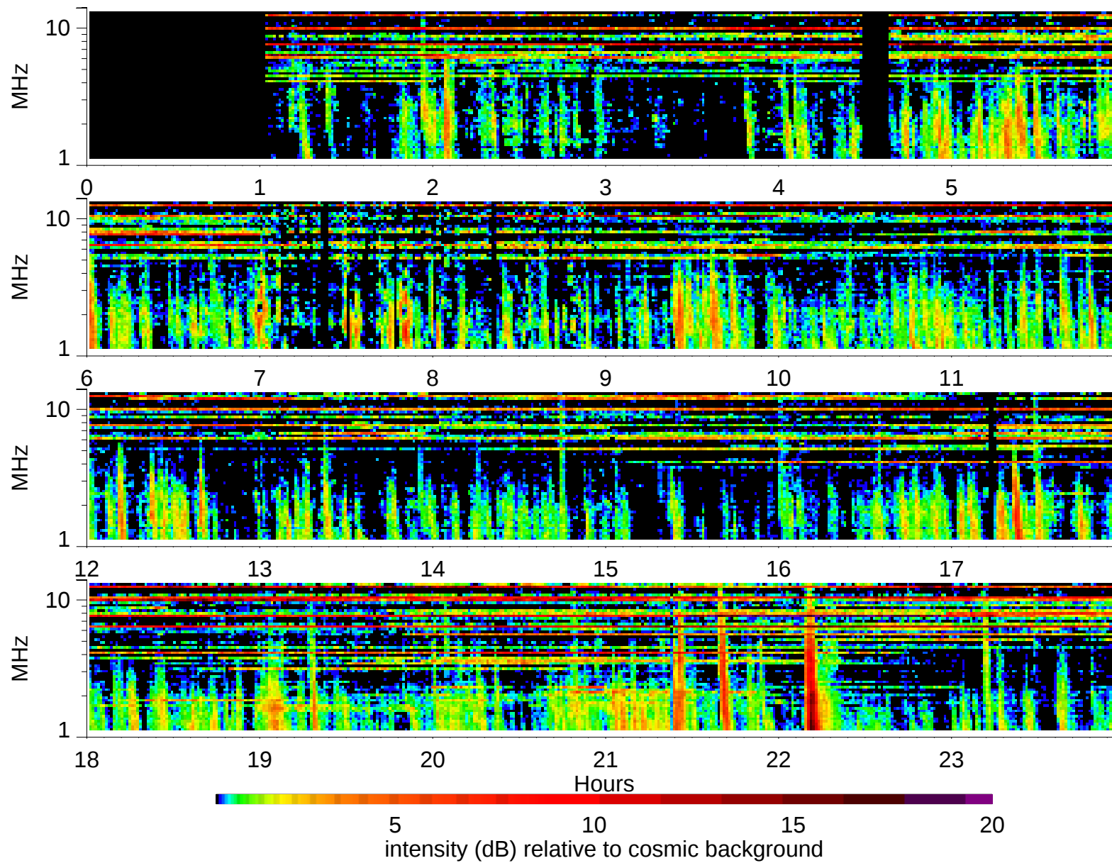
Wind Waves RAD2 receiver: 1999/12/25
